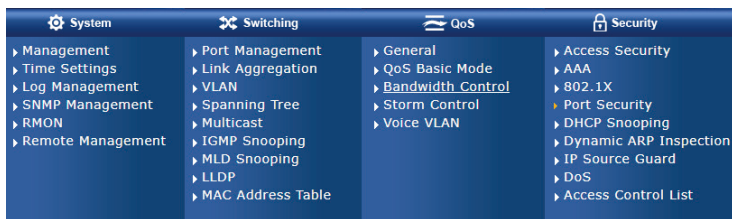
Figure 5-5: Switch Sub-menu
