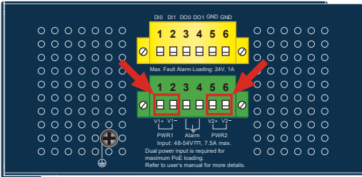
Figure 3-3: IGS-4215-16P2T2S DC Inlet Power Socket
