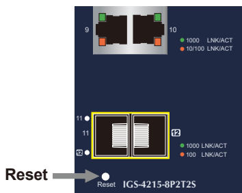
Figure 6-1: IGS-4215 PoE Series Reset Button
