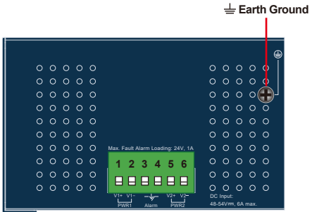
Figure 3-5: Grounding Method (applies to all models)
