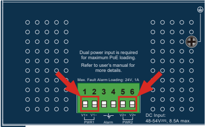
Figure 3-2: IGS-4215-4UP4T2S/IGS-4215-8UP2T2S DC Inlet Power Socket
