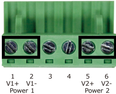
Figure 3-4: Power 1 & 2 Pins of Terminal Block Connector
