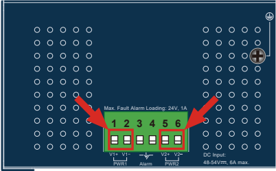
Figure 3-1: IGS-4215-4P4T/IGS-4215-4P4T2S/IGS-4215-8P2T2S DC Inlet Power Socket
